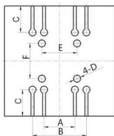
Mould installation
