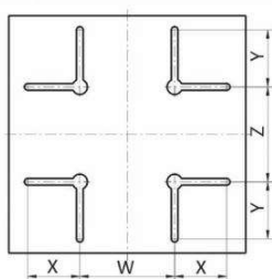
type mould installation drawing
